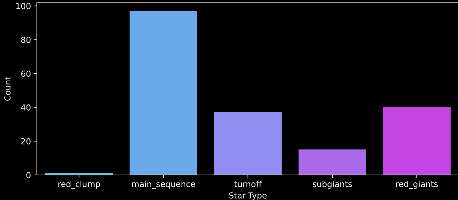
APOGEE DR17 Field: [LMC24] Count plot of Star Type
