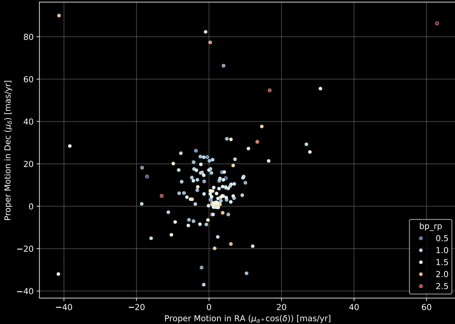
APOGEE DR17 Field: [LMC24] Proper Motion Diagram (n= 190)
