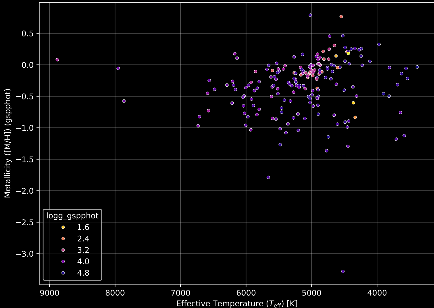
APOGEE DR17 Field: [LMC24] Stellar Population Parameters (n= 190)
