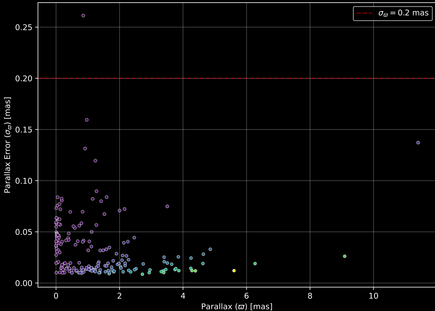
APOGEE DR17 Field: [LMC24] Parallax Quality (n= 190)
