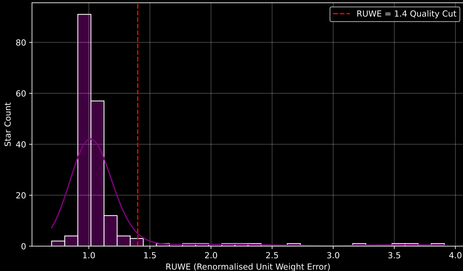
GAPOGEE DR17 Field [LMC24] RUWE Distribution (n= 184)
