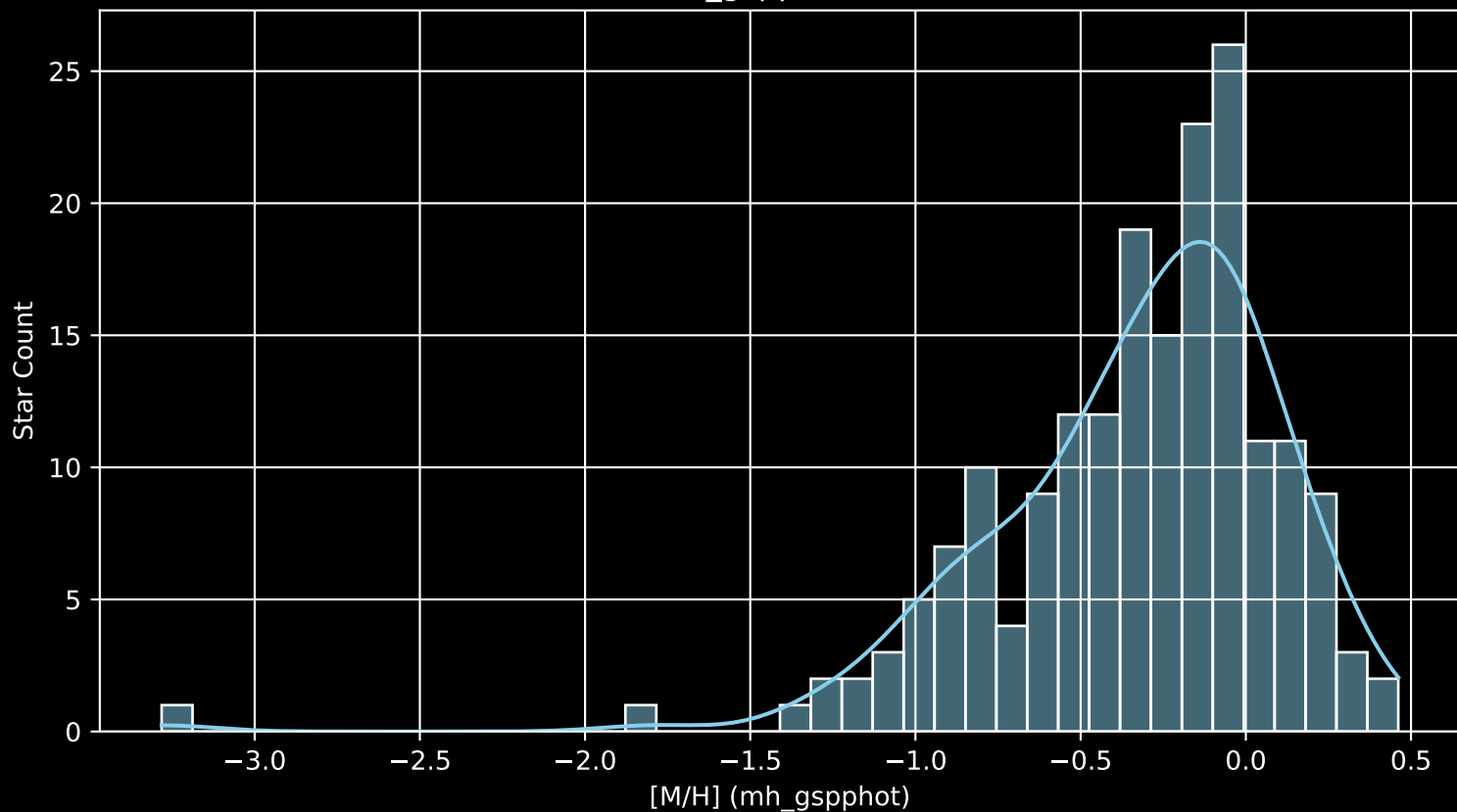
APOGEE DR17 Field: [LMC24 [M/H] (mh_gspphot) (n= 188)
